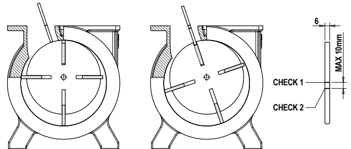
Pic. 6.3 – Vanes check for PN 45-58
