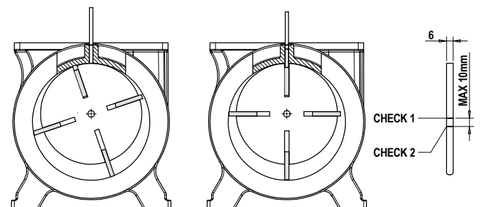
Pic. 6.4 – Vanes check for PN 84-106
