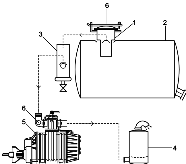
Pic. 4.3 PN pump with standard manifold (above) PN pump with mixer manifold (below)
