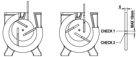
Pic. 6.3 – Vanes check for PN 23-33-40
