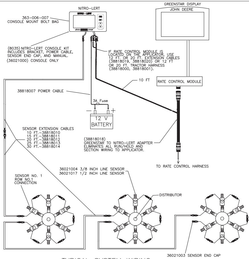
TYPICAL SYSTEM WIRING NITRO-LERT TO GREENSTAR ADAPTER
