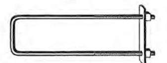
For fastening Truck bodies to chassis or making Hay Racks with heavy sills made of 1/2" round steel with 6" threads, one washer plate and 2 nuts furnished.
