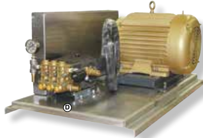
10HP, 15HP or 20HP Pump Units Manufactured by Dultmeier
