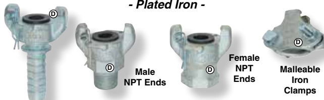
Hose Ends
