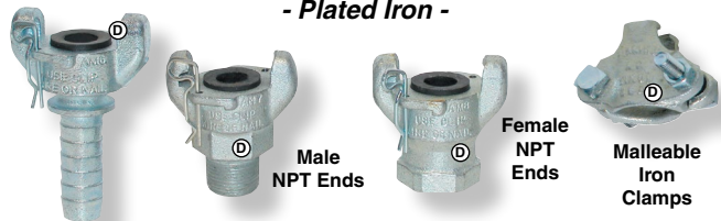
Hose Ends
