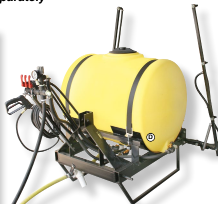
PT200R 3-Point Sprayer (Shown with options: manual controls, handgun kit & boom)
