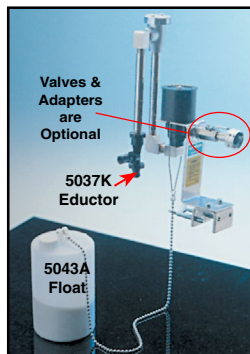
The Hydro-Minder may be easily installed on any liquid reservoir.
